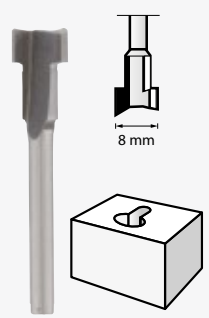
Fresa (HSS) 8,0 mm (655)
