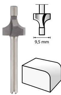
Fresa (HSS) 9,5 mm (615)
